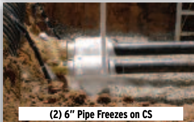
30" X 24" Wet Tap on PCCP
